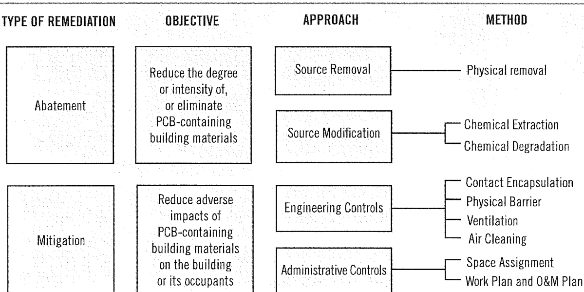
FIGURE 2.1 Framework for Methods to Remediate PCBs in Building Materials
