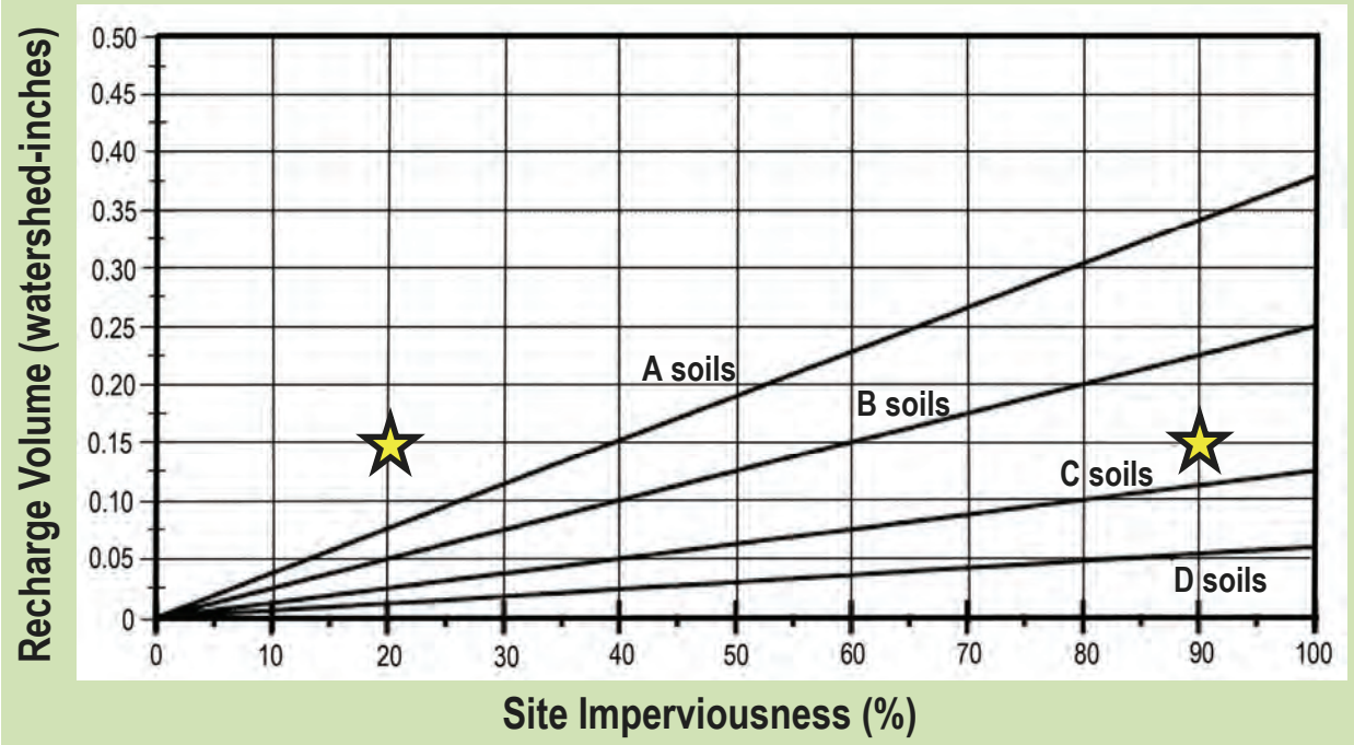
Figure 18. Use the line graph above to plot your site's imperviousness and recharge volume. For example, if your recharge volume equals 0.15 and your site imperviousness equals 20% you are above the minimum recharge volume for all HSG soils. However, if your site imperviousness is 90% you do not meet the minimum recharge volume for HSG A or B soils. Additional small-scale practices may be necessary to achieve the site's recharge volume. Source: Maryland Stormwater Design Manual, "Unified Stormwater Sizing Criteria", p 2.6.
