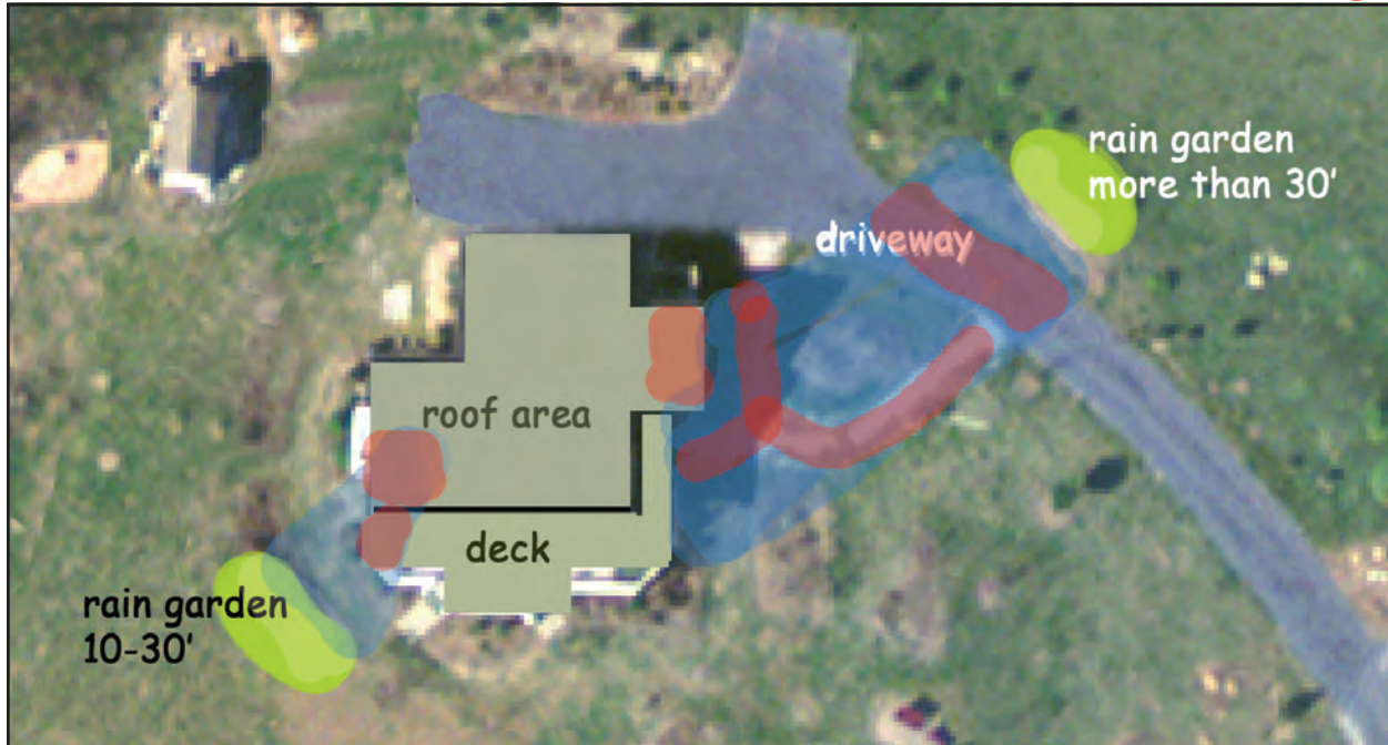
Figure 12: Your drainage area may include impervious surfaces like portions of the lawn (highlighted in blue), roof, sidewalk, and driveway (highlighted in red). These elements can direct more stormwater runoff into rain gardens.
