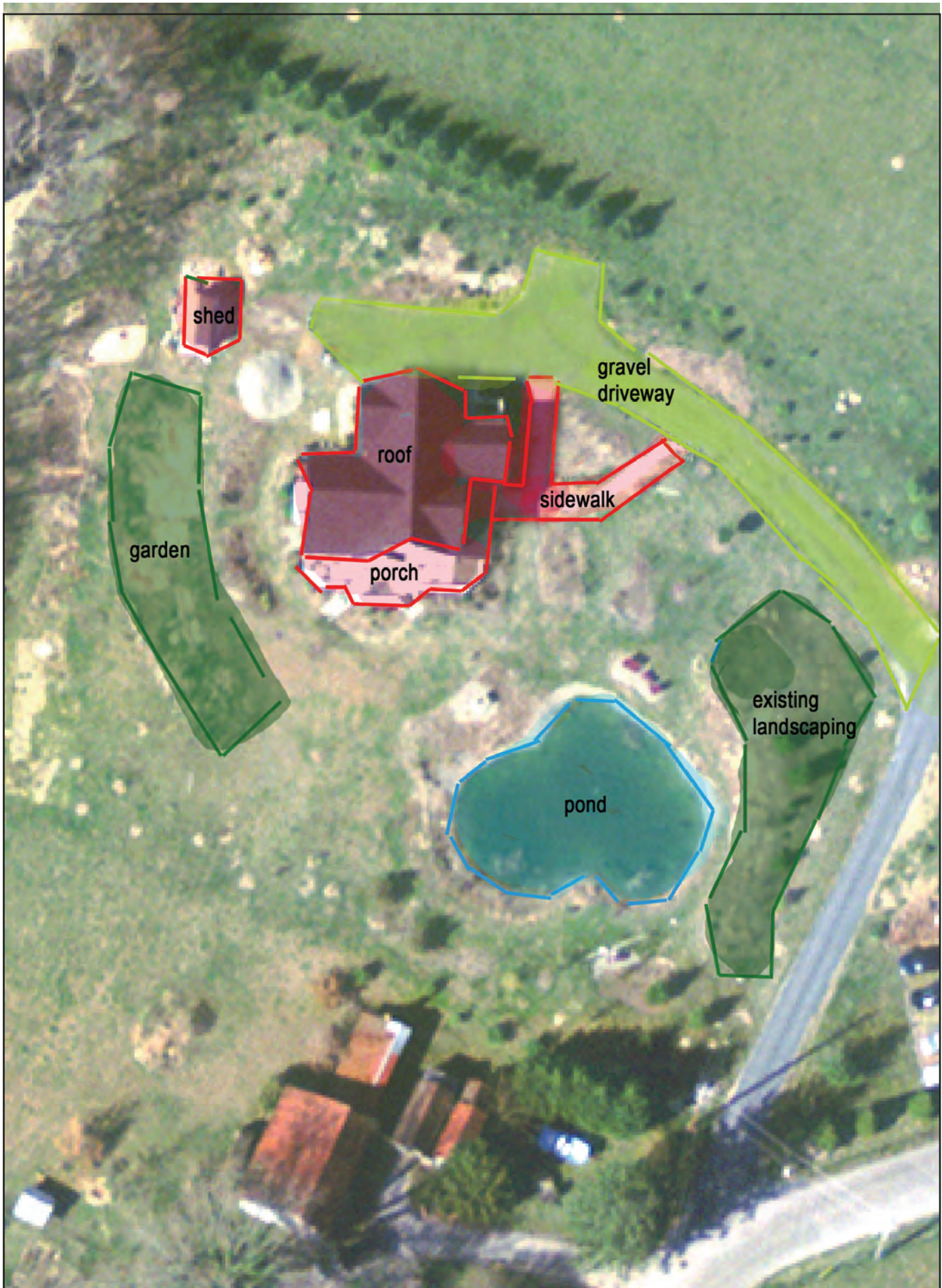
Figure 7. Identify existing landscaping features relative to your house to help locate the best place to build your rain garden. This can help you capture runoff from impervious surfaces and improve your landscape.
